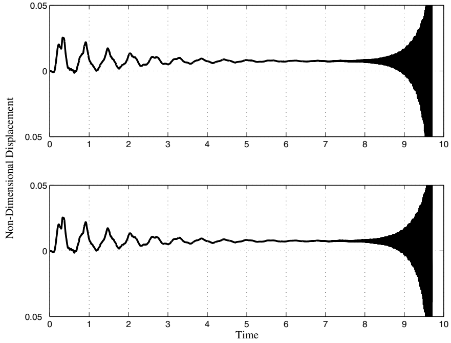
Fig. 16. Legendre-collocation: In-plane displacements at an offset point u(0.29, 0.29, t) (top) and v(0.29, 0.29, t) (bottom). N = 13 , \Delta t = 10^{-6} , h = 0.1 , c = 1.25 , g = 29.60 , Fixed point conv. tolerance 10^{-10} . No filtering was used.
